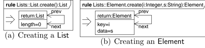
Fig. 2. Transformation rules for creating instances of ListItem
