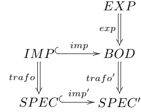
Fig. 2. Transformation semantics
